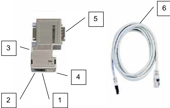
Abbildung 1: ACCON-NetLink-PRO compact
